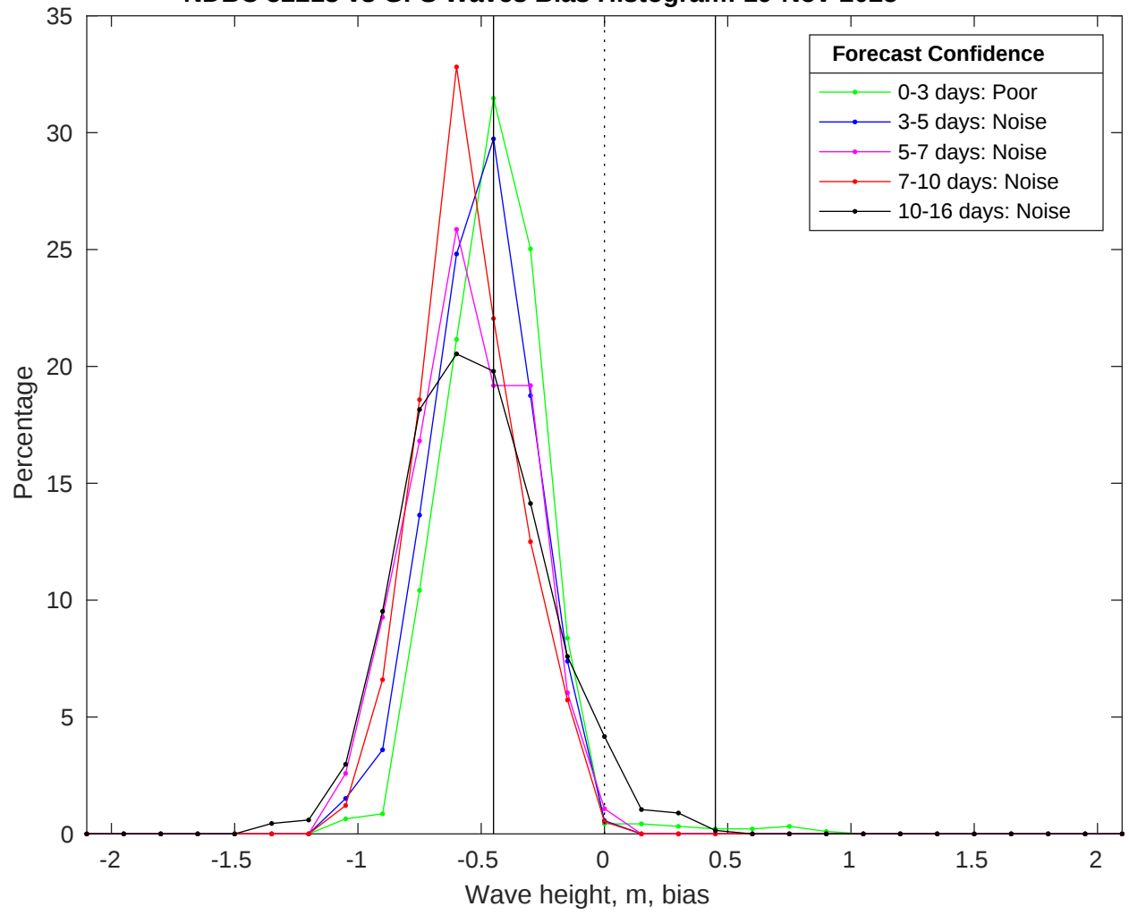
NDBC 52213 vs GFS Waves Bias Histogram: 19-Nov-2025
