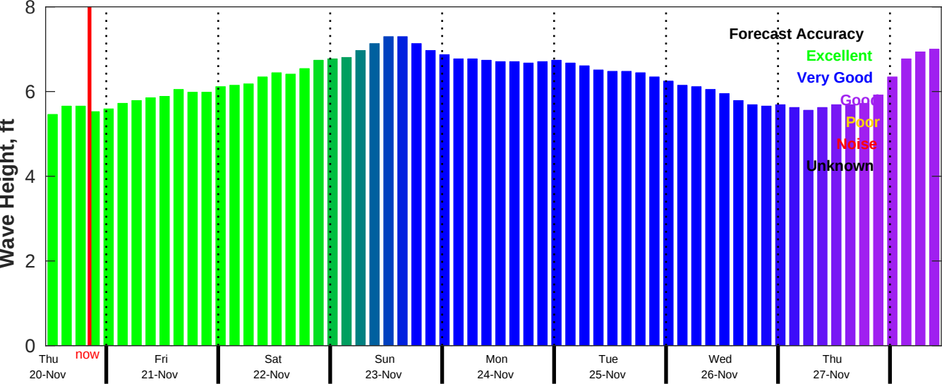
CMEMS Wave Forecast for NDBC 52213 from 19-Nov-2025 11:00:00 to 27-Nov-2025 11:00:00
