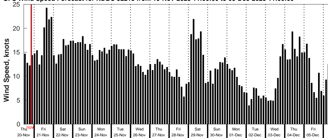
GFS Wind Speed Forecast for NDBC 52213 from 19-Nov-2025 11:00:00 to 05-Dec-2025 11:00:00
