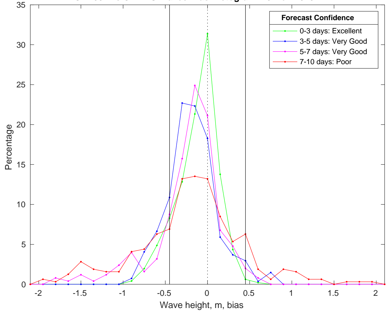
NDBC 41004 vs CMEMS Waves Bias Histogram: 20-Nov-2025
