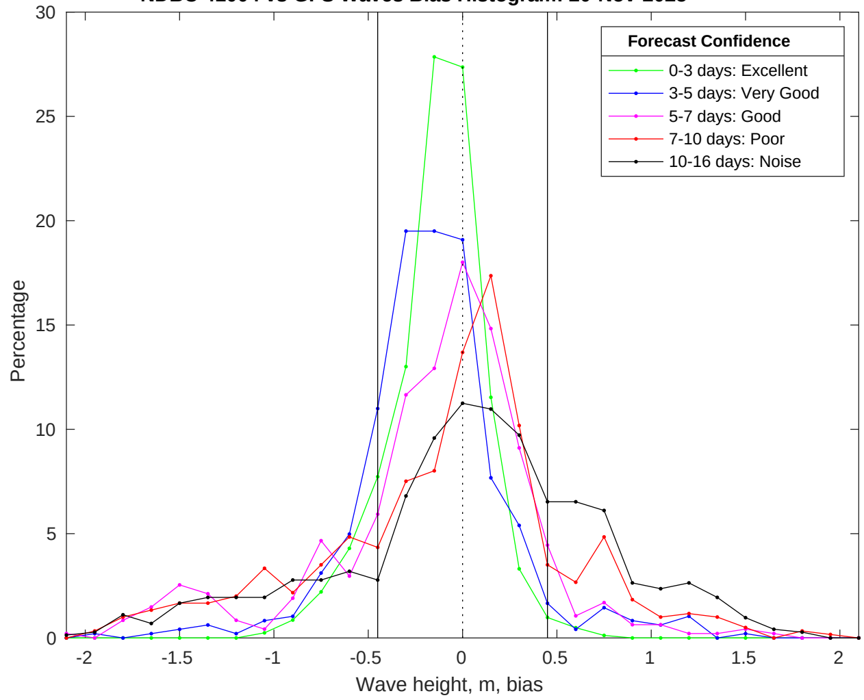
NDBC 41004 vs GFS Waves Bias Histogram: 20-Nov-2025
