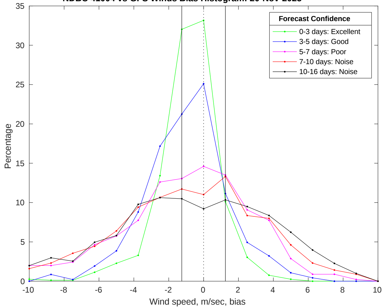
NDBC 41004 vs GFS Winds Bias Histogram: 20-Nov-2025
