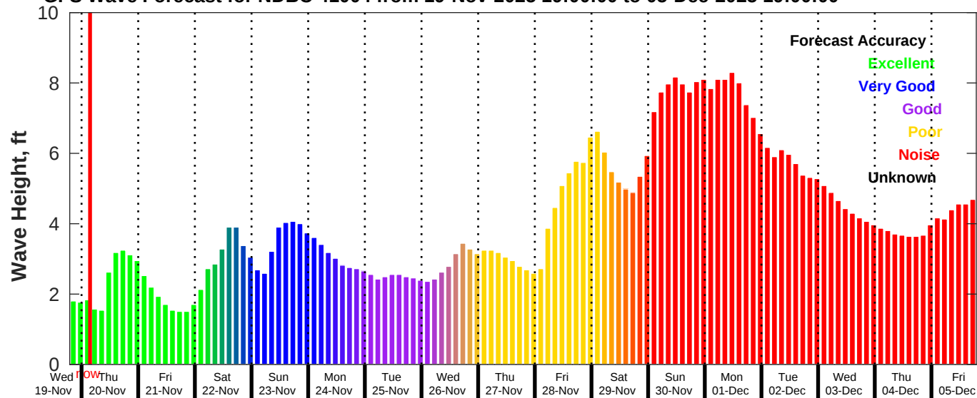
GFS Wave Forecast for NDBC 41004 from 19-Nov-2025 19:00:00 to 05-Dec-2025 19:00:00
