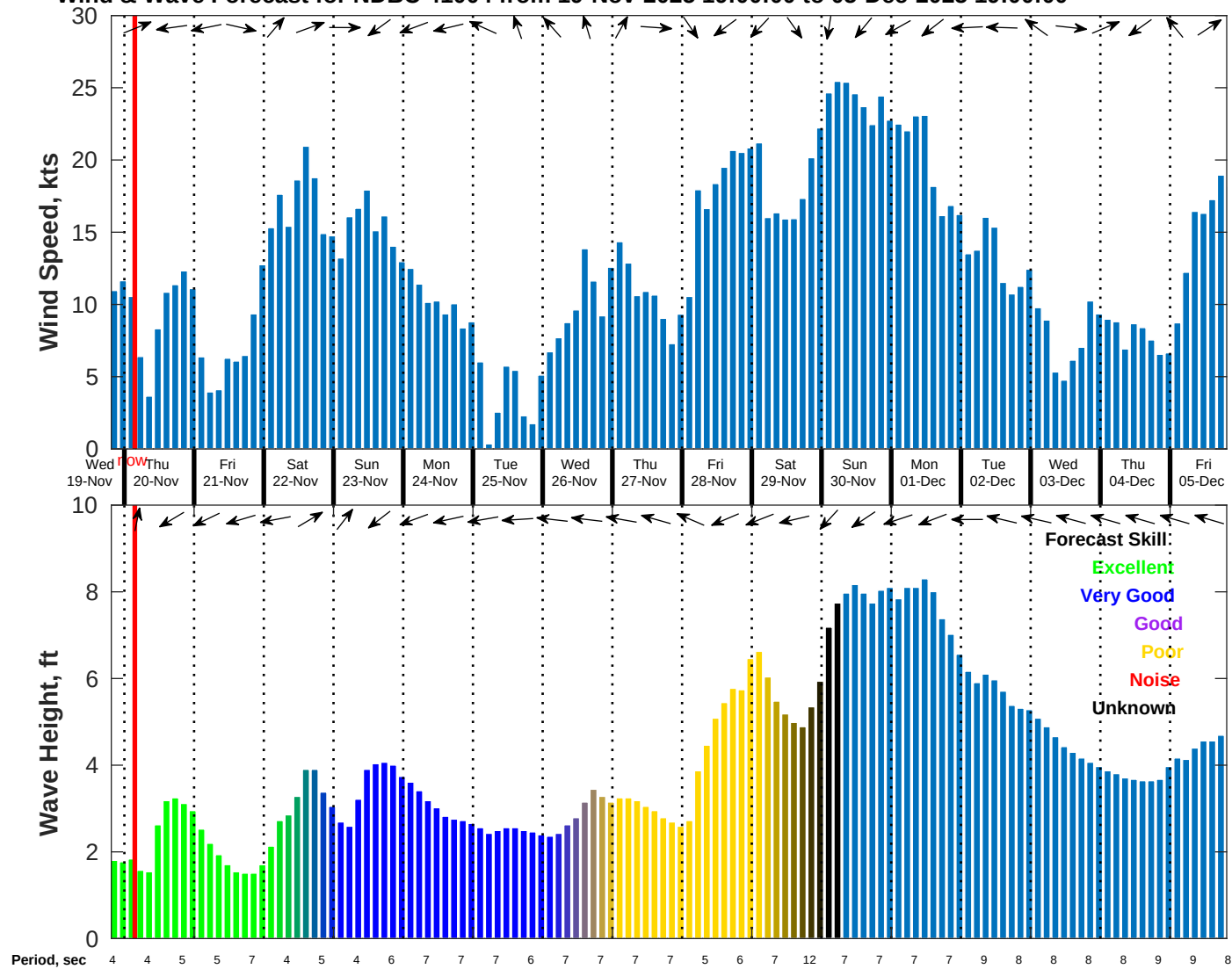
Wind & Wave Forecast for NDBC 41004 from 19-Nov-2025 19:00:00 to 05-Dec-2025 19:00:00
