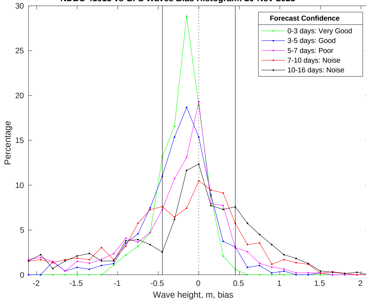
NDBC 41013 vs GFS Waves Bias Histogram: 20-Nov-2025
