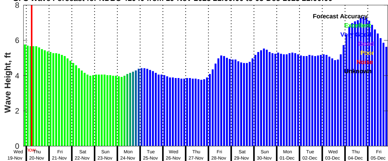
GFS Wave Forecast for NDBC 41040 from 19-Nov-2025 21:00:00 to 05-Dec-2025 21:00:00
