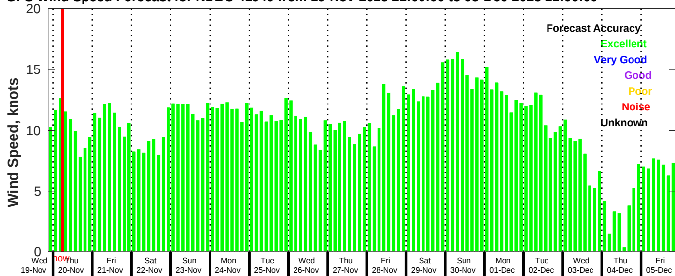
GFS Wind Speed Forecast for NDBC 41040 from 19-Nov-2025 21:00:00 to 05-Dec-2025 21:00:00
