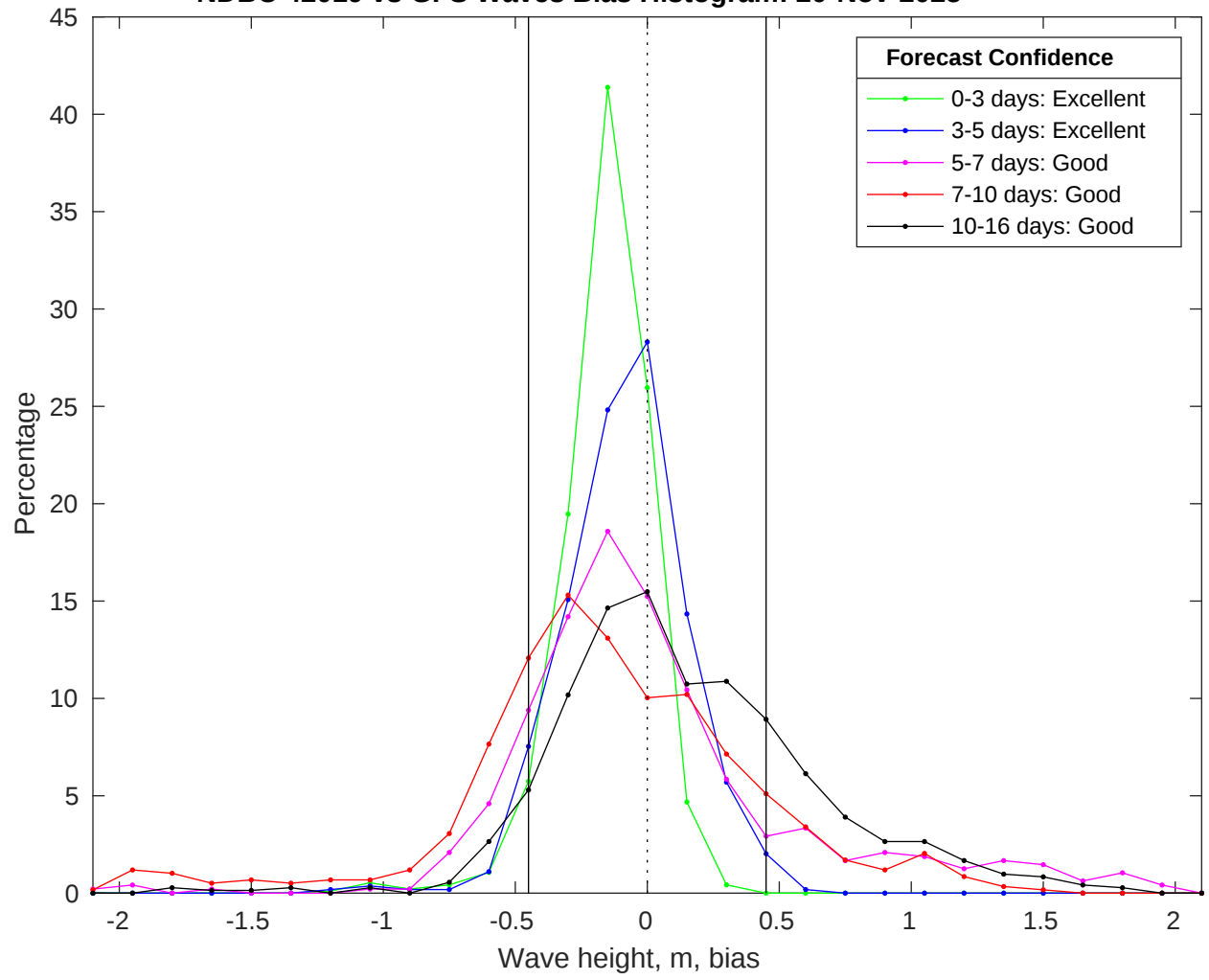
NDBC 42019 vs GFS Waves Bias Histogram: 20-Nov-2025
