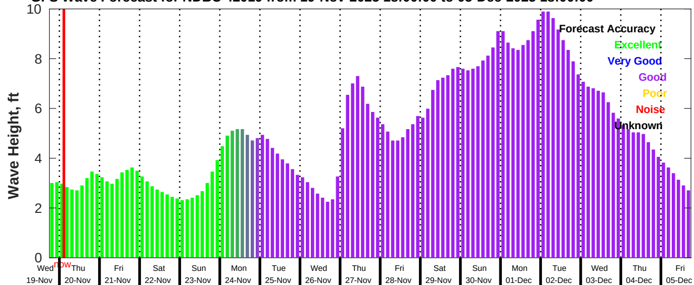
GFS Wave Forecast for NDBC 42019 from 19-Nov-2025 18:00:00 to 05-Dec-2025 18:00:00
