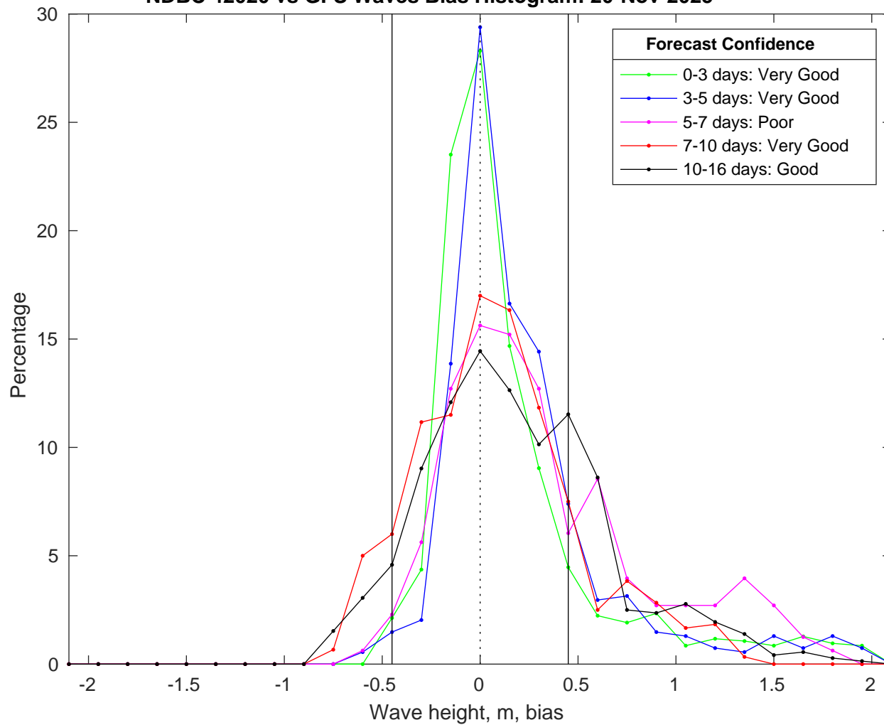
NDBC 42020 vs GFS Waves Bias Histogram: 20-Nov-2025
