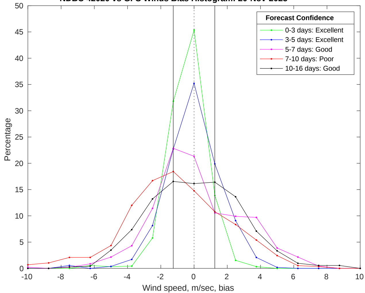
NDBC 42020 vs GFS Winds Bias Histogram: 20-Nov-2025
