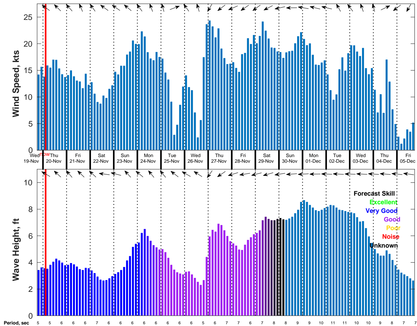
Wind & Wave Forecast for NDBC 42020 from 19-Nov-2025 18:00:00 to 05-Dec-2025 18:00:00
