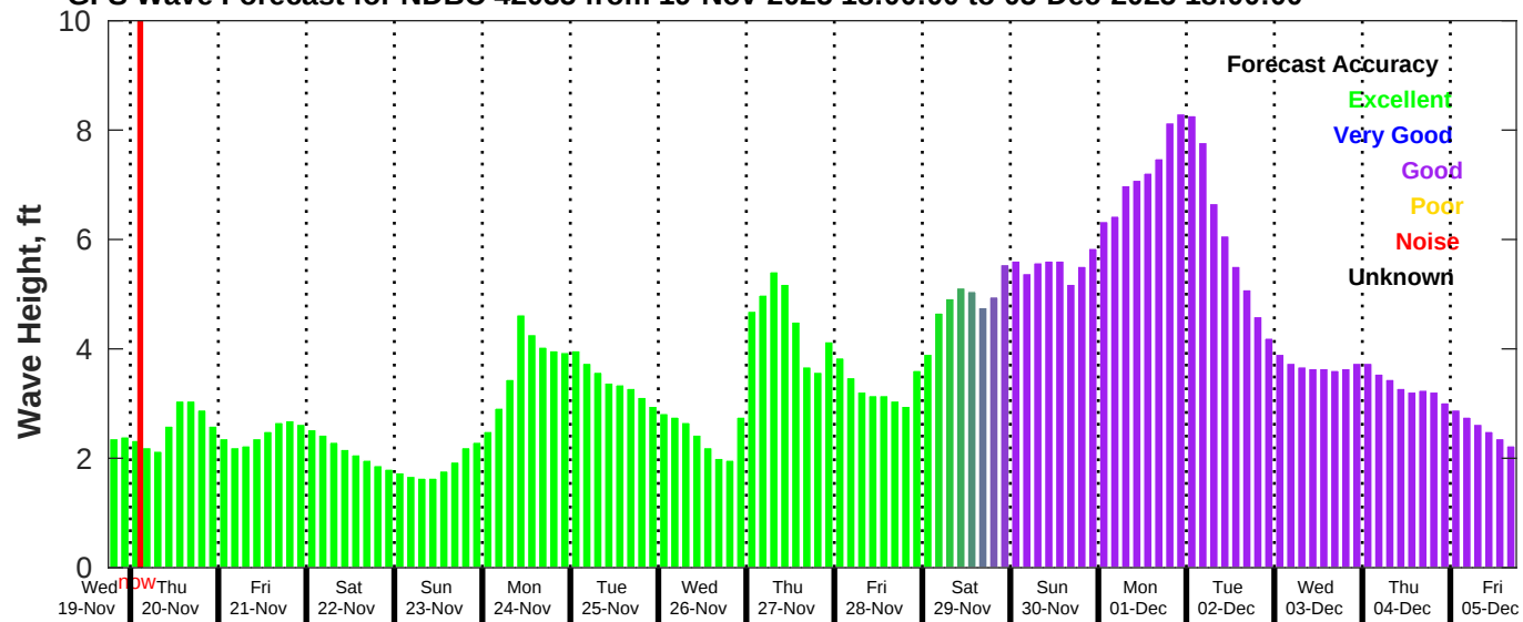
GFS Wave Forecast for NDBC 42035 from 19-Nov-2025 18:00:00 to 05-Dec-2025 18:00:00
