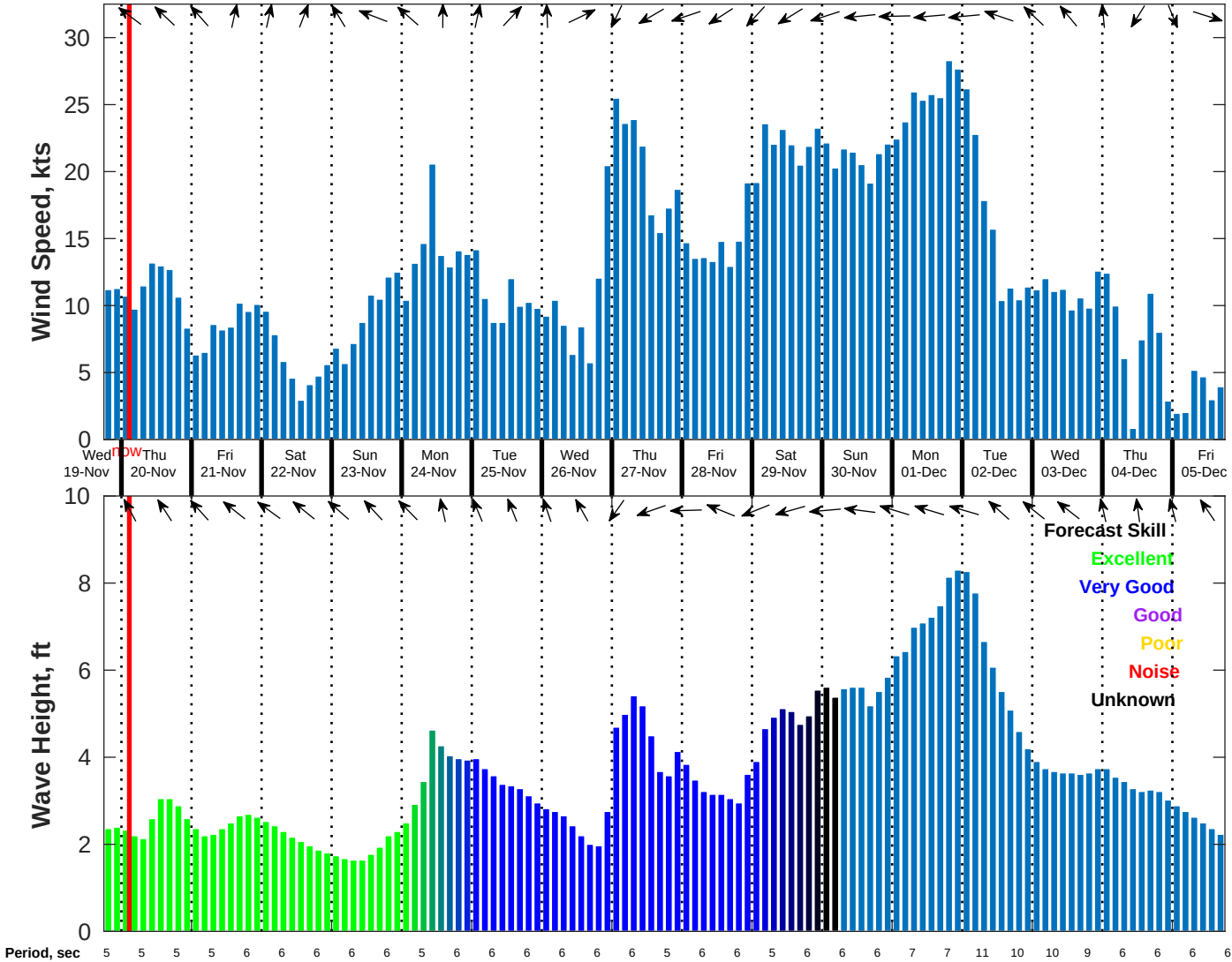
Wind & Wave Forecast for NDBC 42035 from 19-Nov-2025 18:00:00 to 05-Dec-2025 18:00:00
