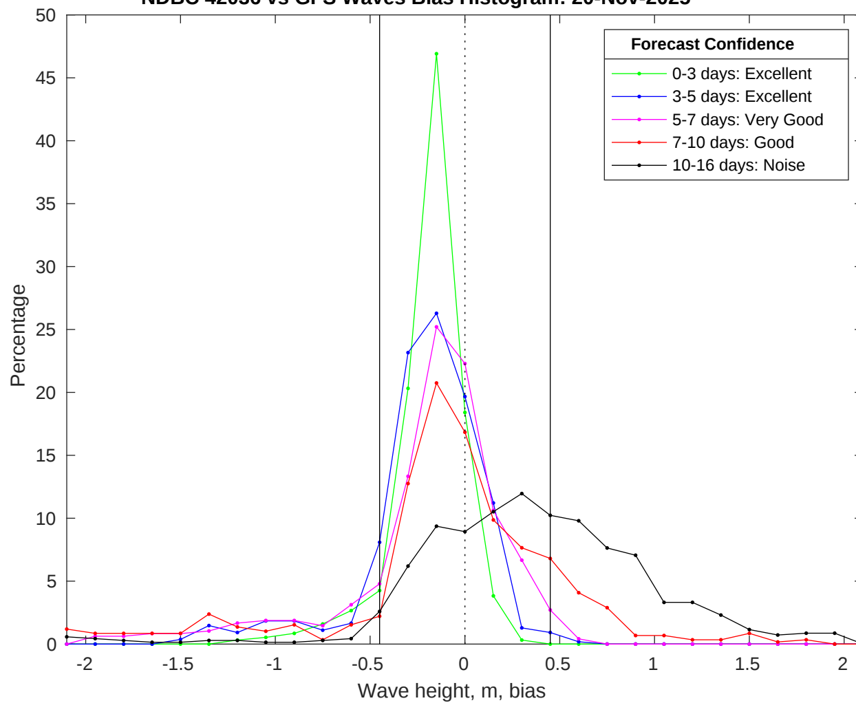
NDBC 42036 vs GFS Waves Bias Histogram: 20-Nov-2025
