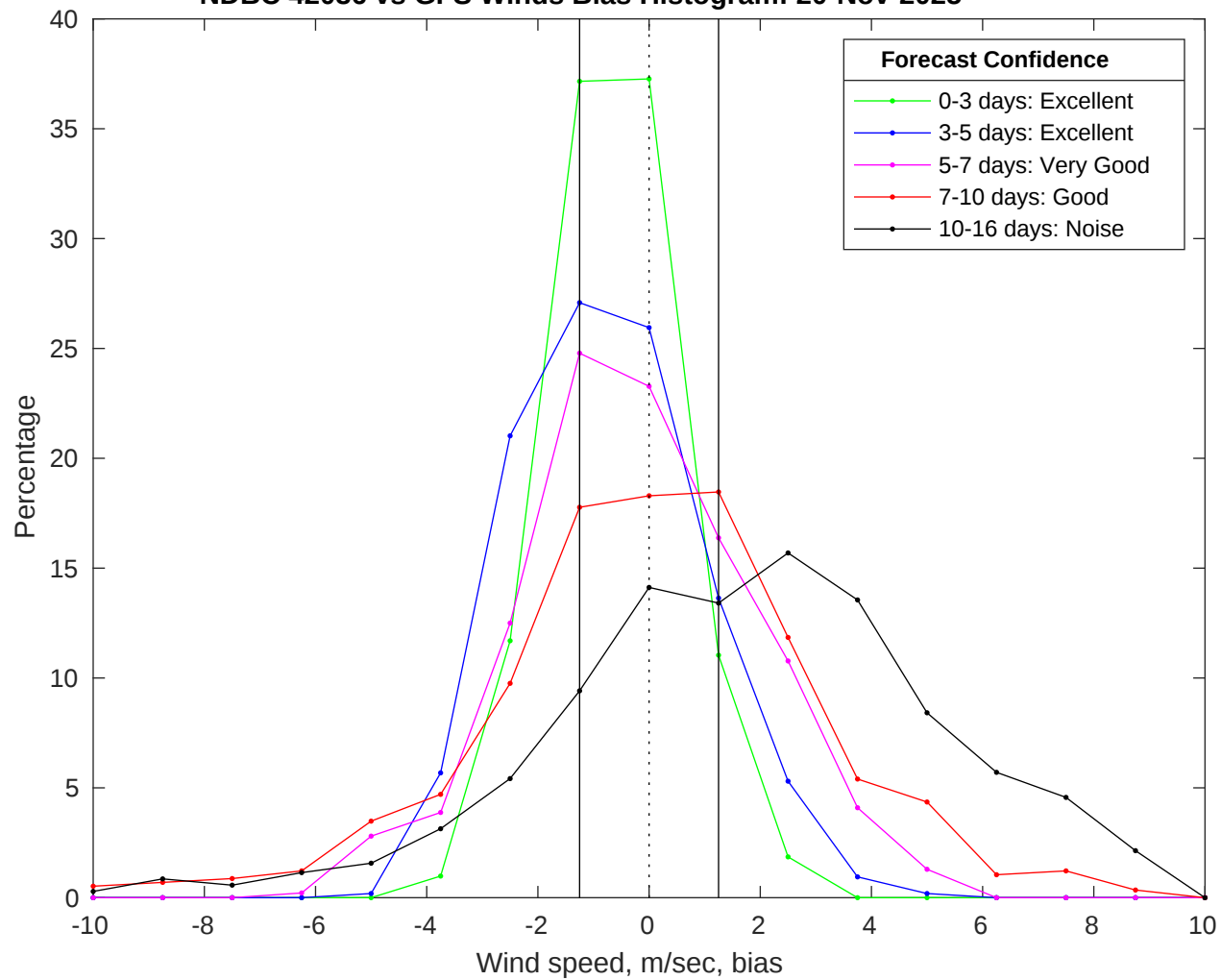
NDBC 42036 vs GFS Winds Bias Histogram: 20-Nov-2025
