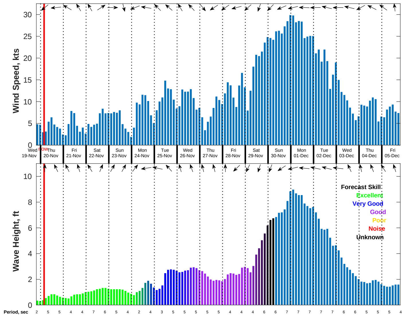
Wind & Wave Forecast for NDBC 42036 from 19-Nov-2025 19:00:00 to 05-Dec-2025 19:00:00
