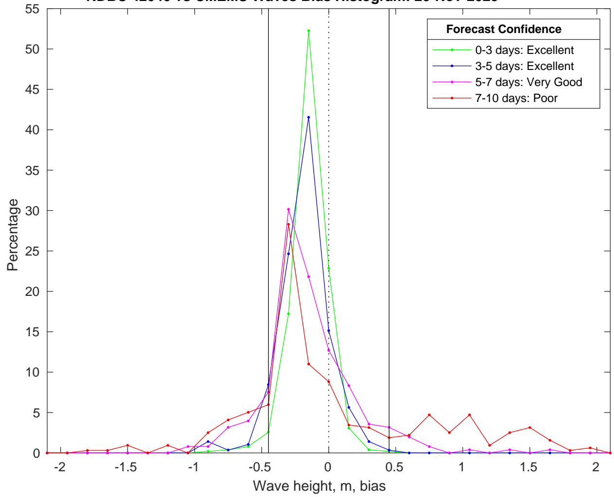
NDBC 42040 vs CMEMS Waves Bias Histogram: 20-Nov-2025
