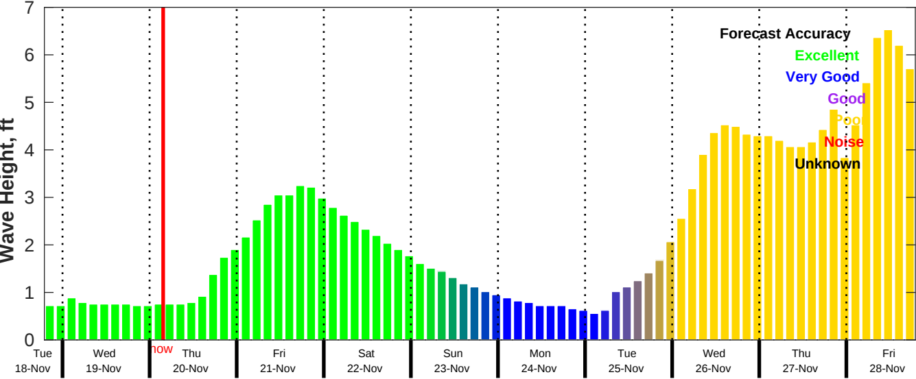
CMEMS Wave Forecast for NDBC 42040 from 18-Nov-2025 19:00:00 to 28-Nov-2025 19:00:00
