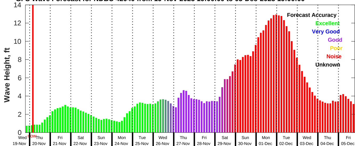
GFS Wave Forecast for NDBC 42040 from 19-Nov-2025 19:00:00 to 05-Dec-2025 19:00:00
