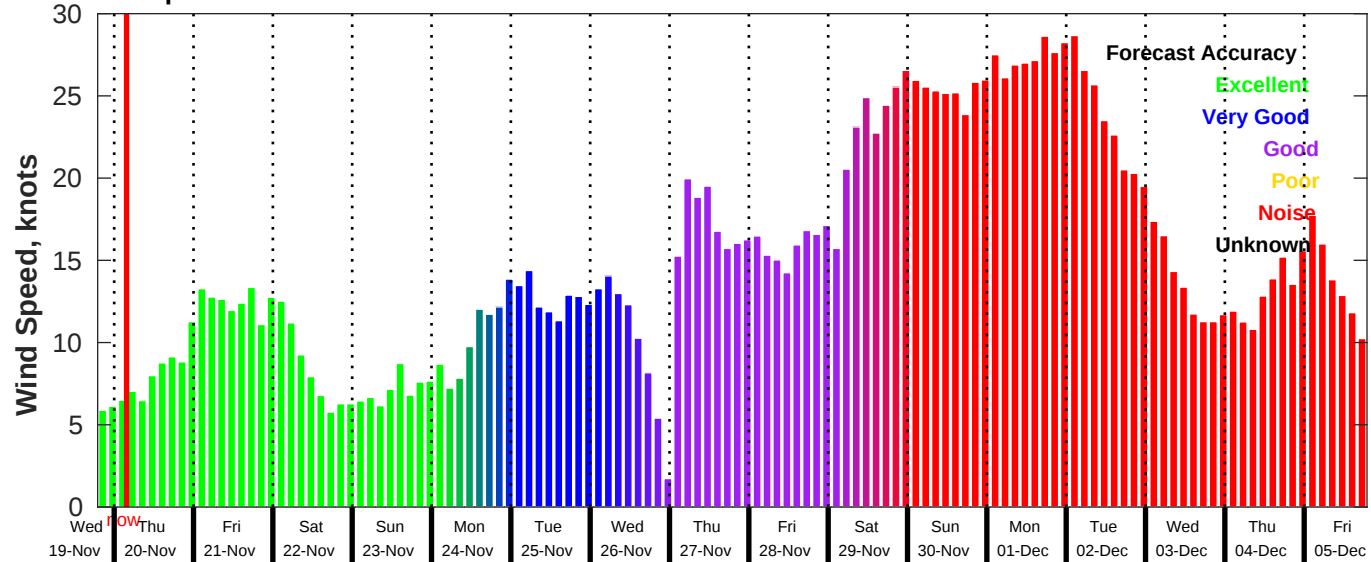
GFS Wind Speed Forecast for NDBC 42040 from 19-Nov-2025 19:00:00 to 05-Dec-2025 19:00:00
