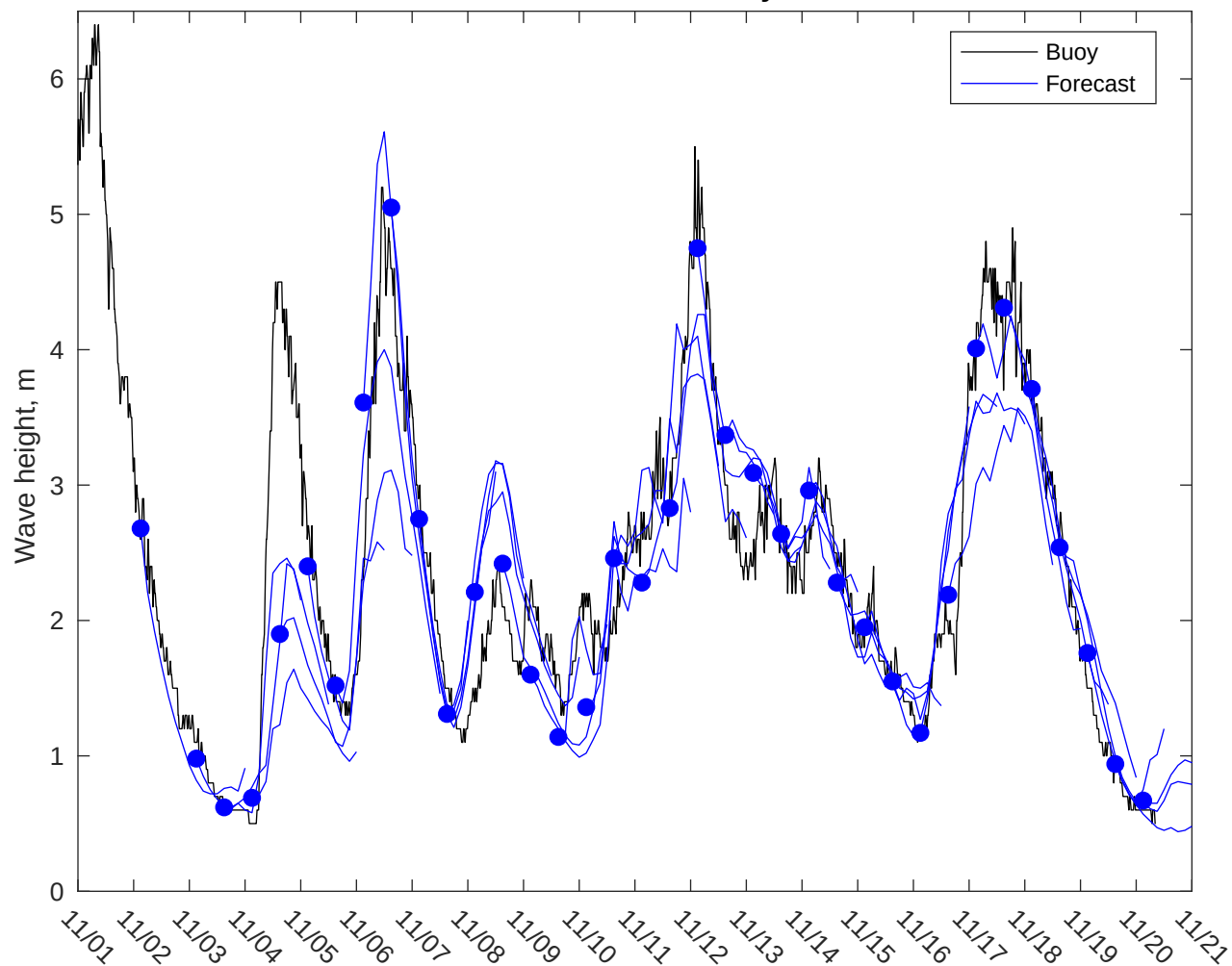
NDBC 44008 vs GFS Waves: 3 to 5 day forecast
