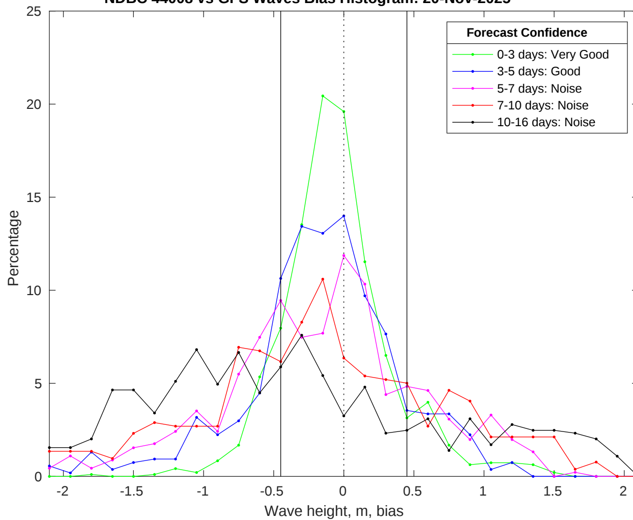
NDBC 44008 vs GFS Waves Bias Histogram: 20-Nov-2025
