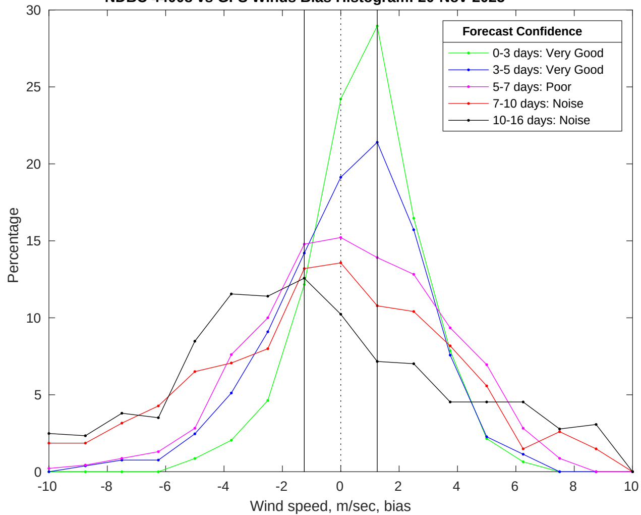
NDBC 44008 vs GFS Winds Bias Histogram: 20-Nov-2025
