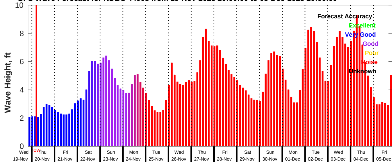
GFS Wave Forecast for NDBC 44008 from 19-Nov-2025 20:00:00 to 05-Dec-2025 20:00:00
