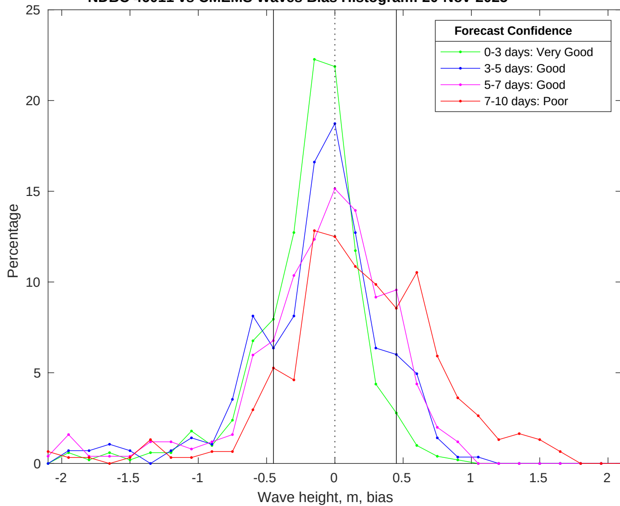
NDBC 46011 vs CMEMS Waves Bias Histogram: 20-Nov-2025
