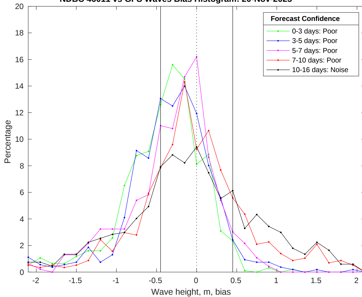
NDBC 46011 vs GFS Waves Bias Histogram: 20-Nov-2025
