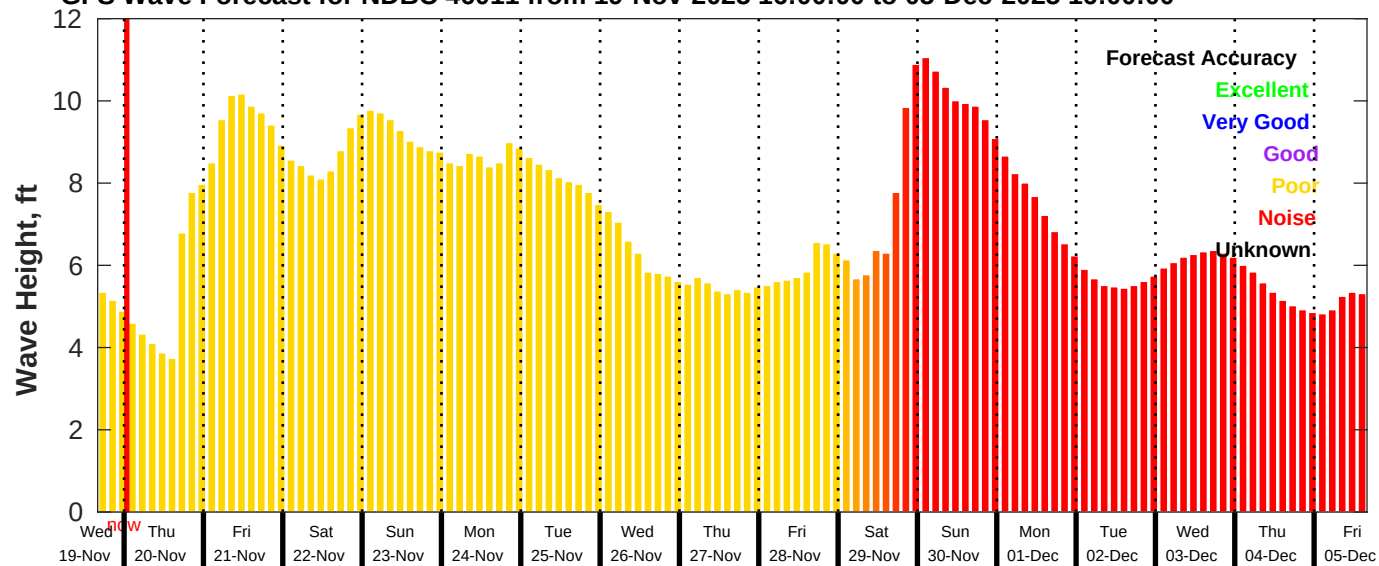
GFS Wave Forecast for NDBC 46011 from 19-Nov-2025 16:00:00 to 05-Dec-2025 16:00:00
