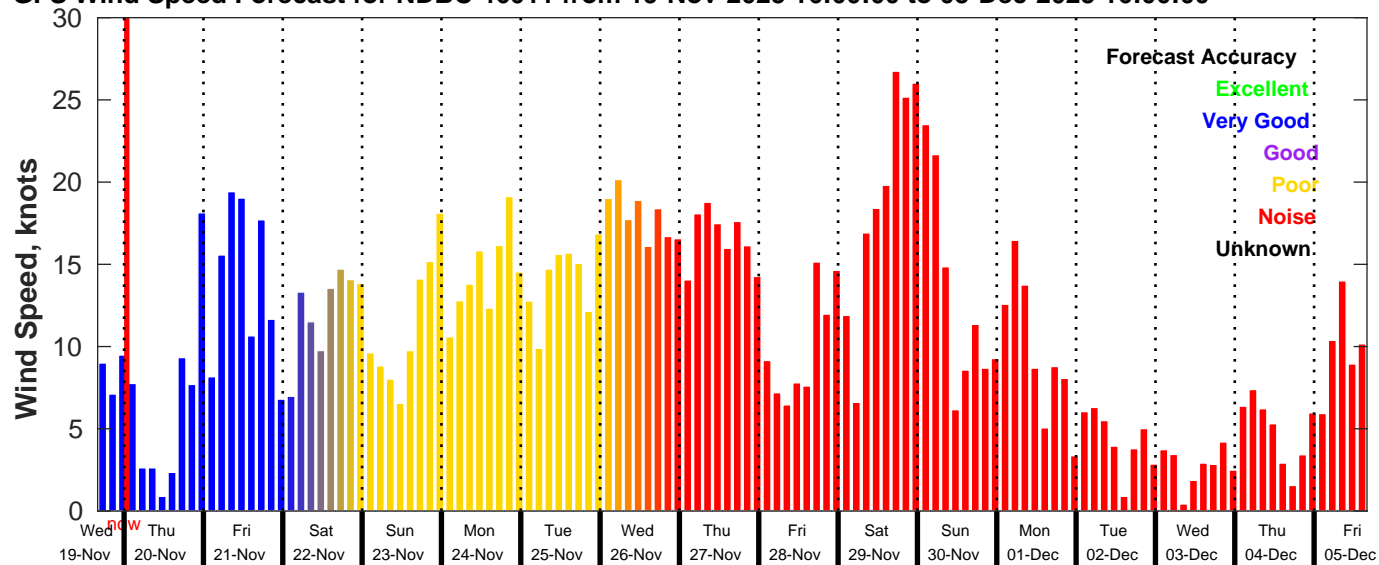
GFS Wind Speed Forecast for NDBC 46011 from 19-Nov-2025 16:00:00 to 05-Dec-2025 16:00:00
