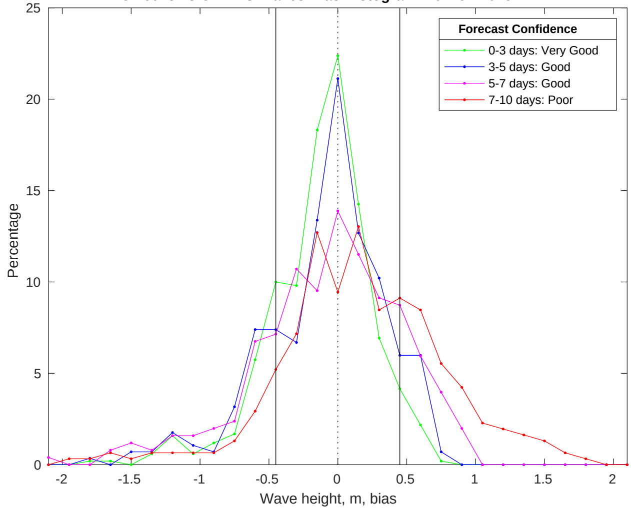
NDBC 46028 vs CMEMS Waves Bias Histogram: 20-Nov-2025
