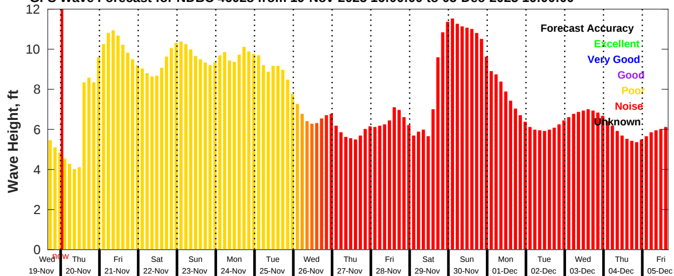
GFS Wave Forecast for NDBC 46028 from 19-Nov-2025 16:00:00 to 05-Dec-2025 16:00:00
