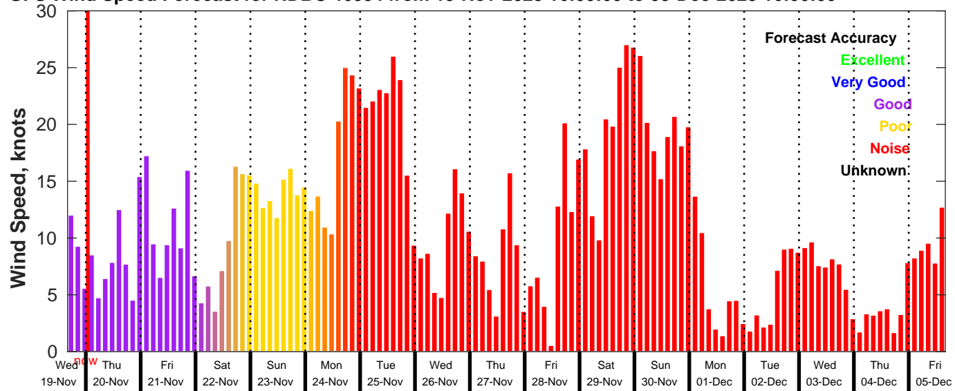
GFS Wind Speed Forecast for NDBC 46054 from 19-Nov-2025 16:00:00 to 05-Dec-2025 16:00:00
