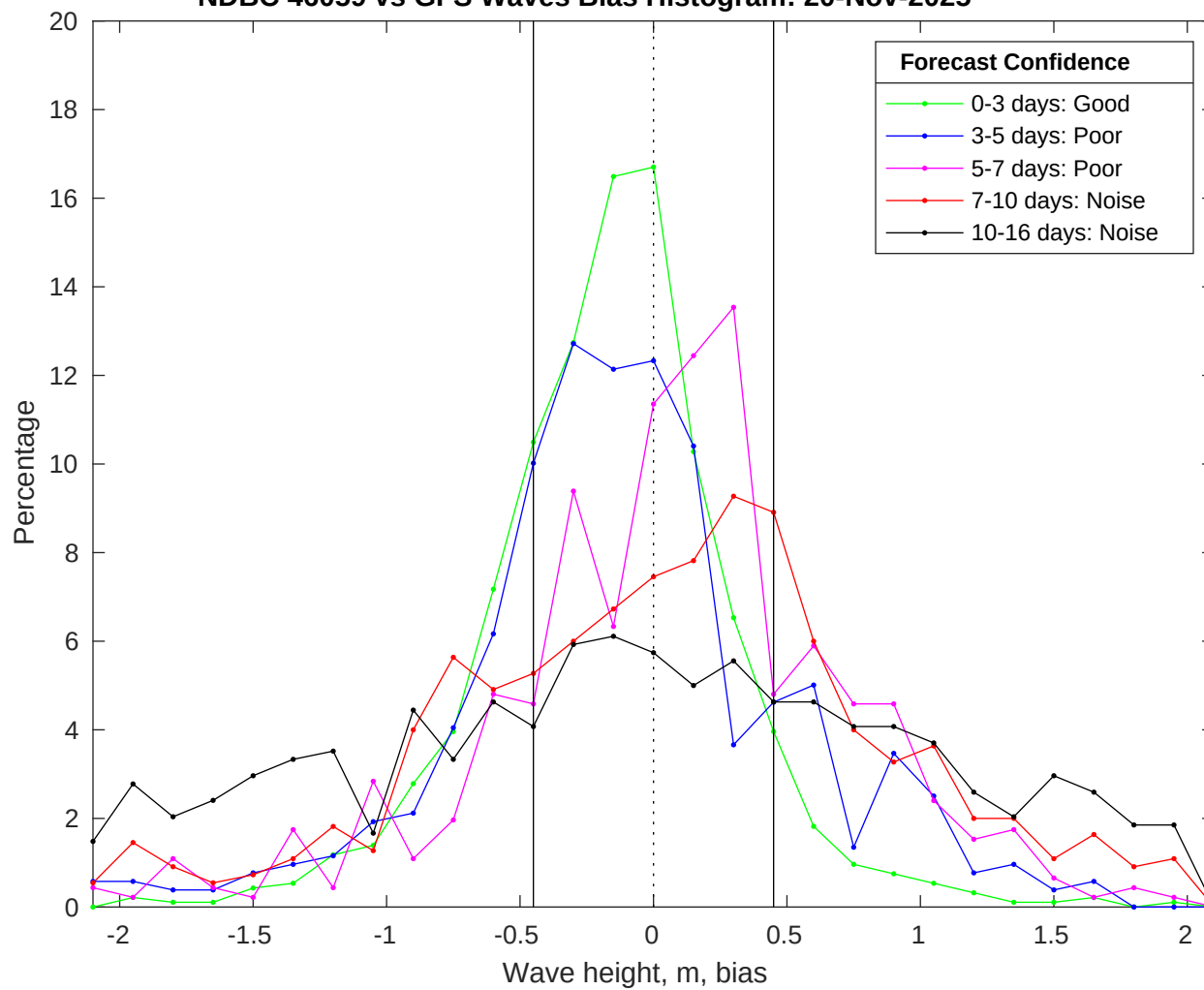
NDBC 46059 vs GFS Waves Bias Histogram: 20-Nov-2025
