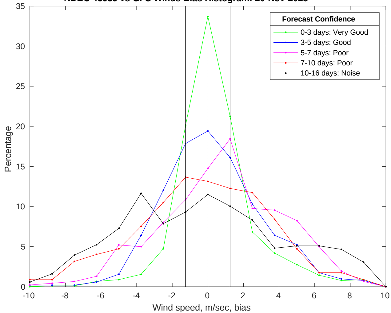
NDBC 46059 vs GFS Winds Bias Histogram: 20-Nov-2025
