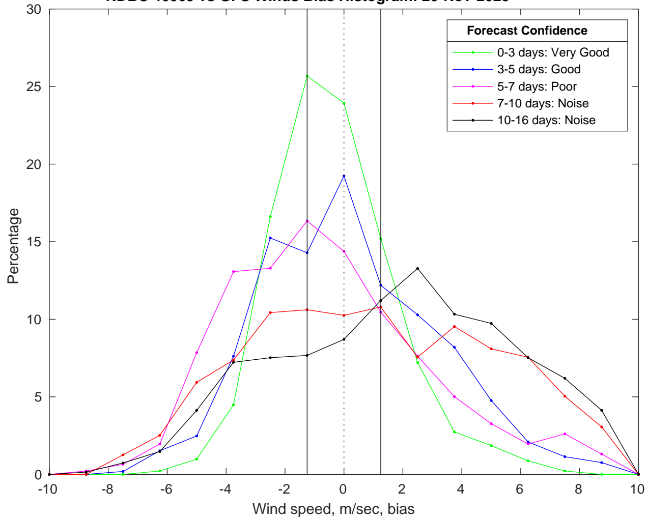
NDBC 46069 vs GFS Winds Bias Histogram: 20-Nov-2025
