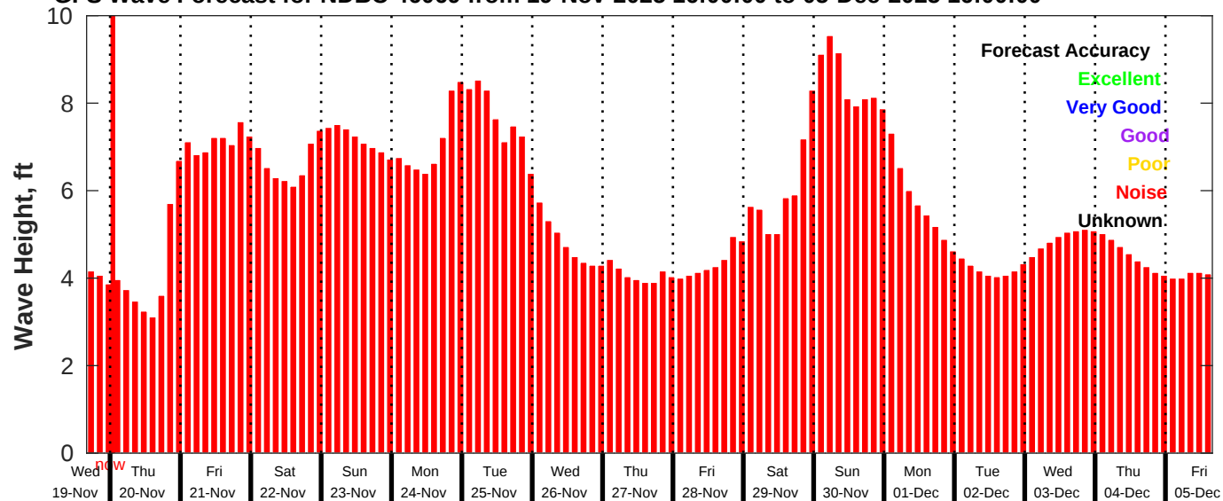
GFS Wave Forecast for NDBC 46069 from 19-Nov-2025 16:00:00 to 05-Dec-2025 16:00:00
