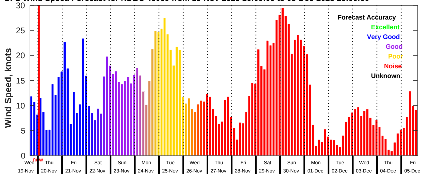
GFS Wind Speed Forecast for NDBC 46069 from 19-Nov-2025 16:00:00 to 05-Dec-2025 16:00:00
