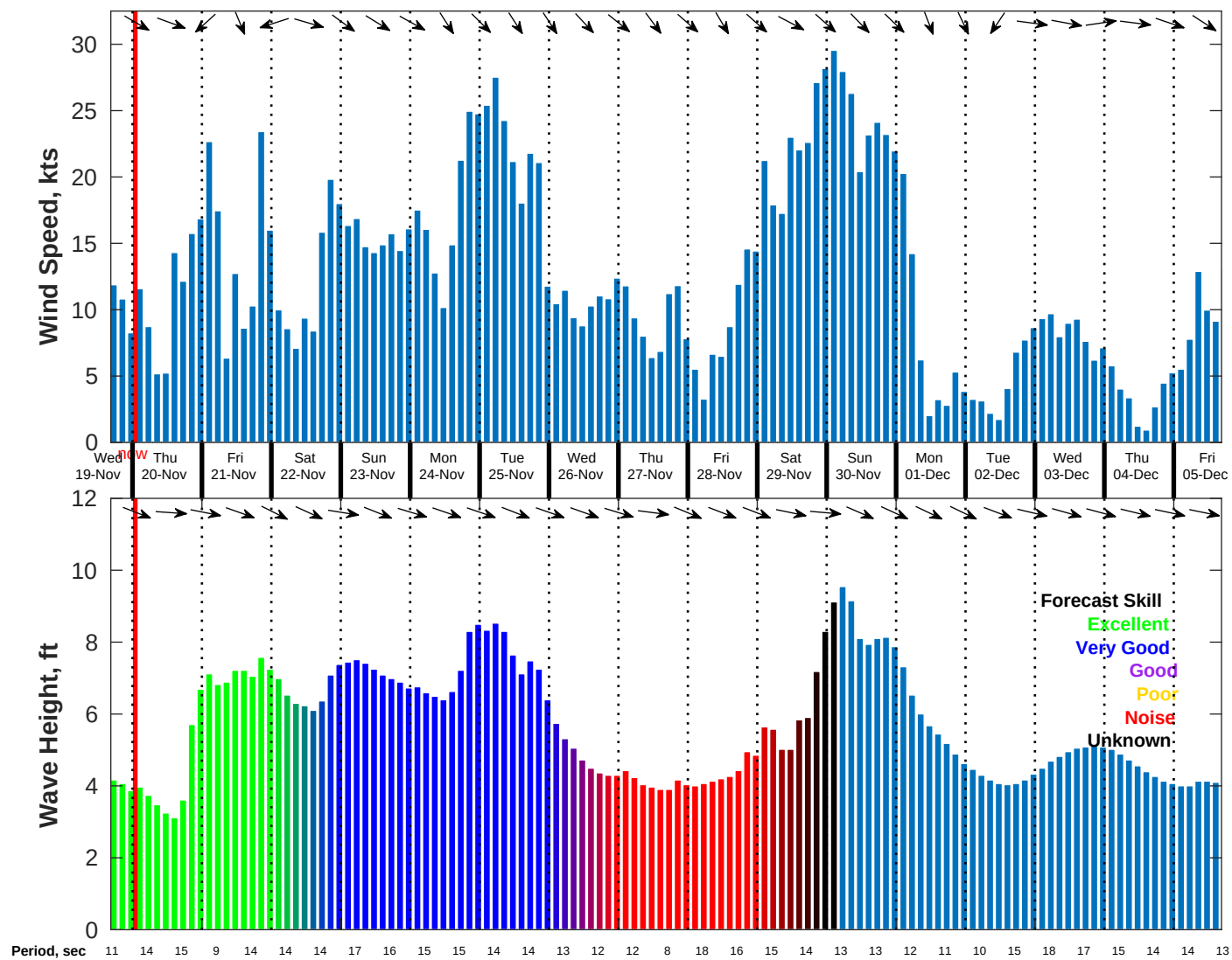
Wind & Wave Forecast for NDBC 46069 from 19-Nov-2025 16:00:00 to 05-Dec-2025 16:00:00
