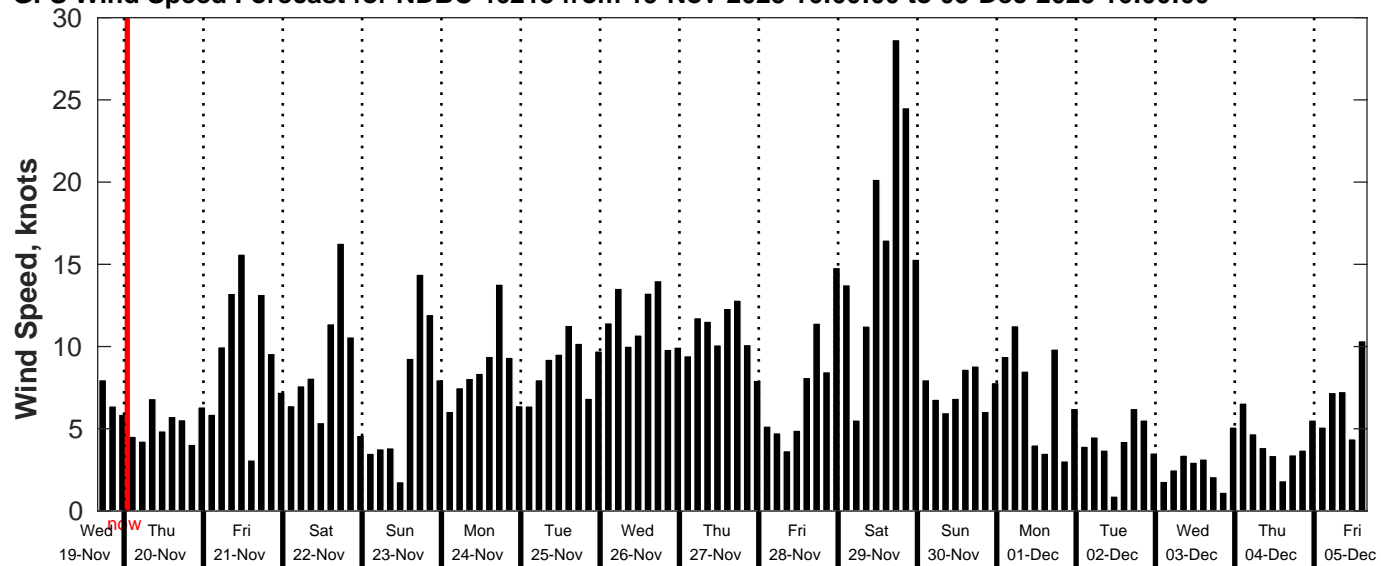
GFS Wind Speed Forecast for NDBC 46215 from 19-Nov-2025 16:00:00 to 05-Dec-2025 16:00:00
