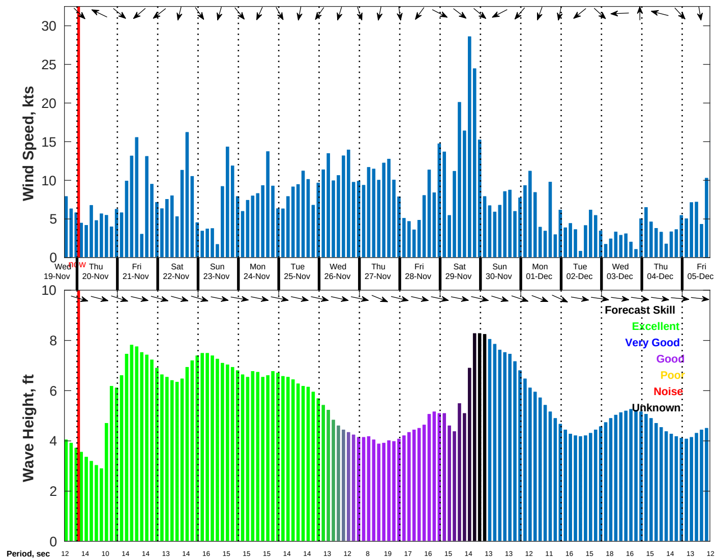
Wind & Wave Forecast for NDBC 46215 from 19-Nov-2025 16:00:00 to 05-Dec-2025 16:00:00
