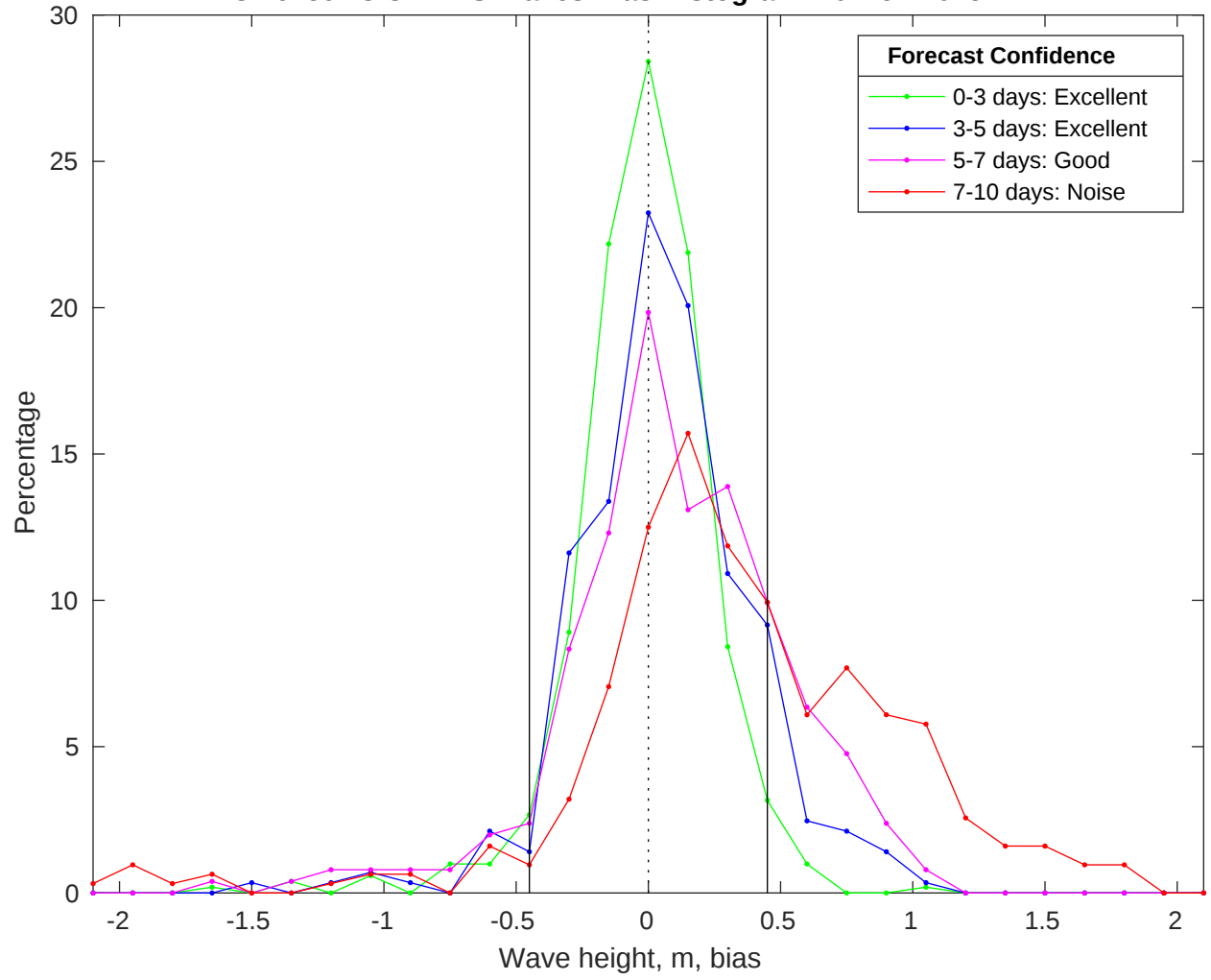
NDBC 46259 vs CMEMS Waves Bias Histogram: 20-Nov-2025
