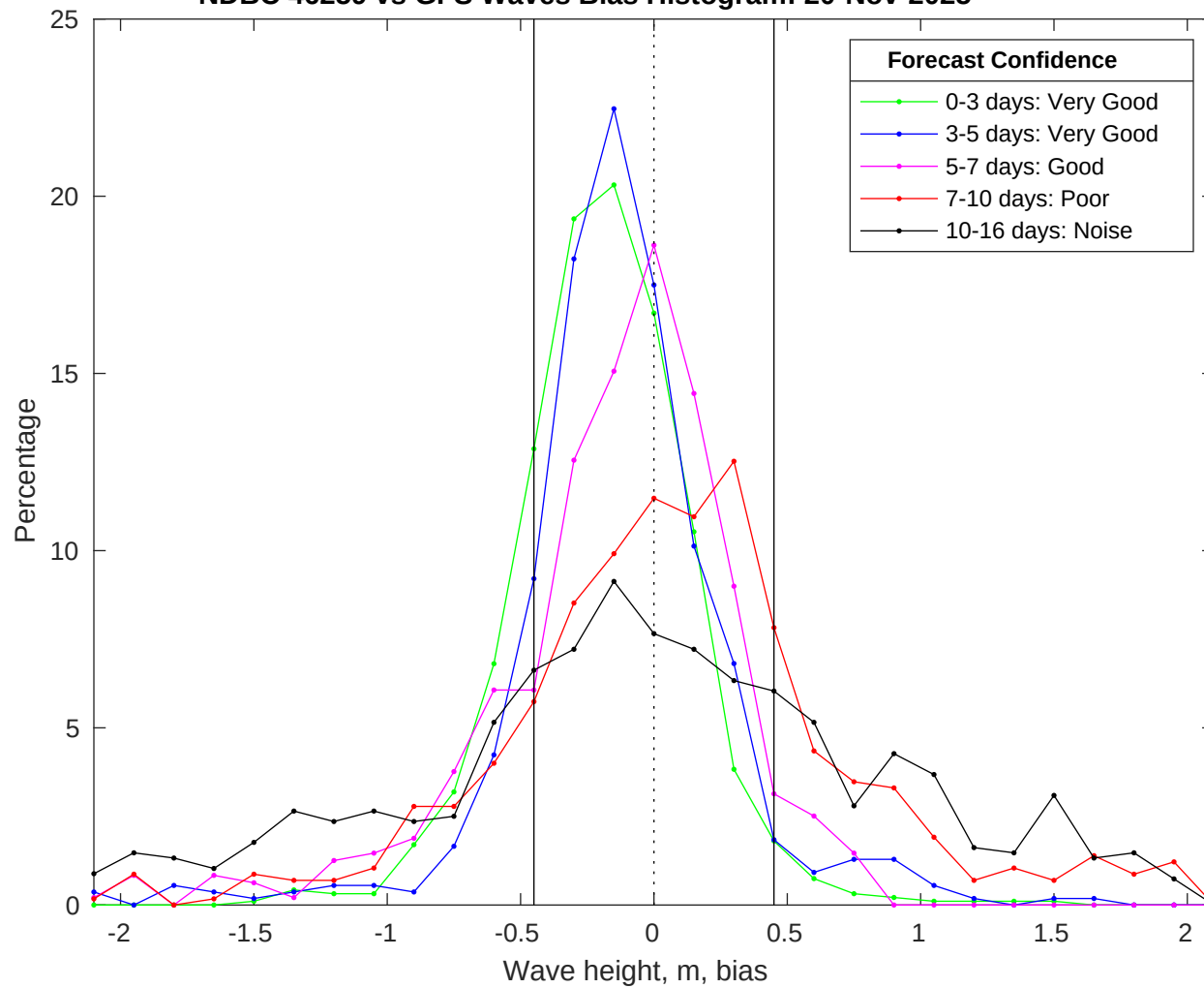
NDBC 46259 vs GFS Waves Bias Histogram: 20-Nov-2025
