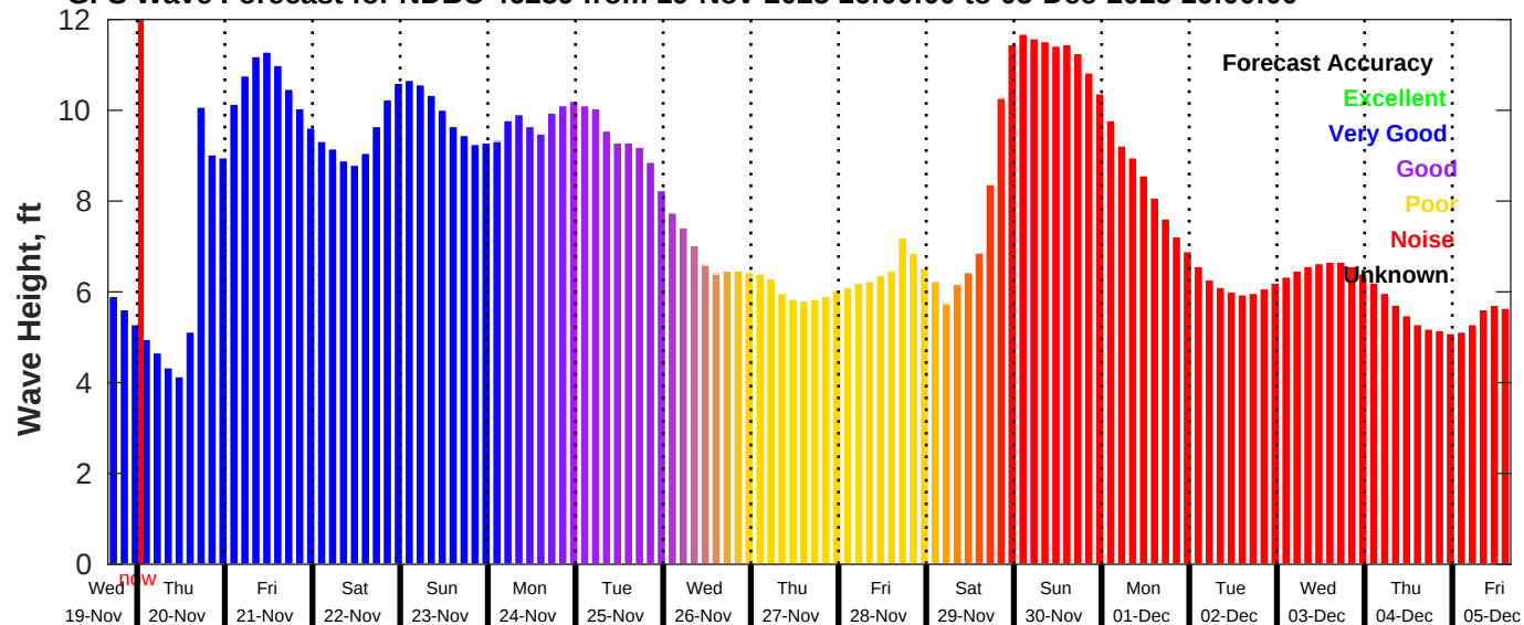
GFS Wave Forecast for NDBC 46259 from 19-Nov-2025 16:00:00 to 05-Dec-2025 16:00:00
