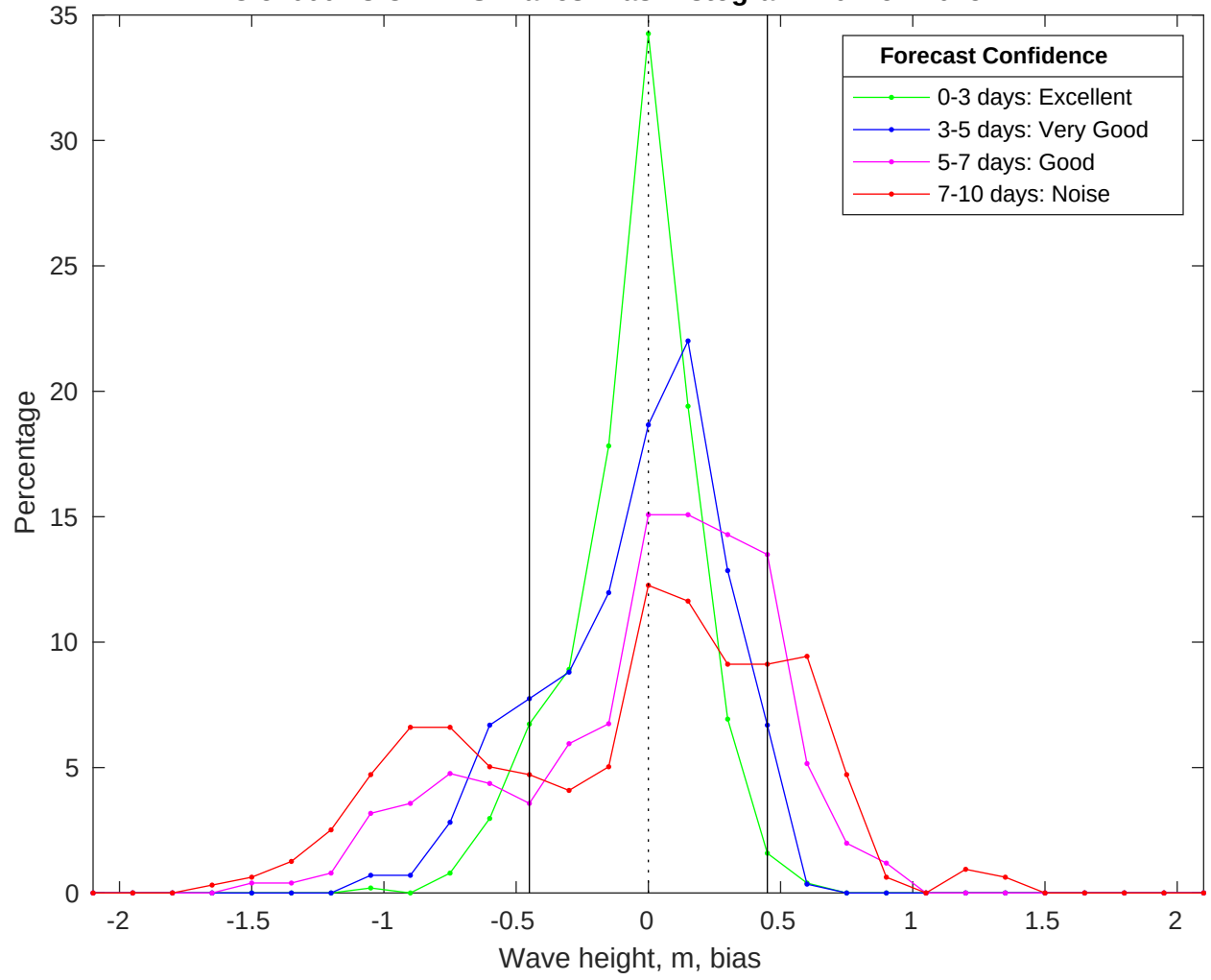
NDBC 51000 vs CMEMS Waves Bias Histogram: 20-Nov-2025
