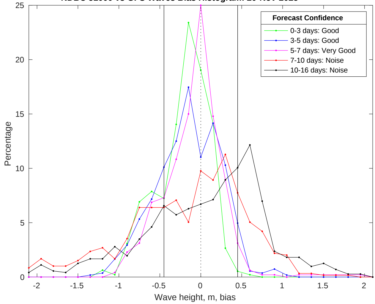
NDBC 51000 vs GFS Waves Bias Histogram: 20-Nov-2025
