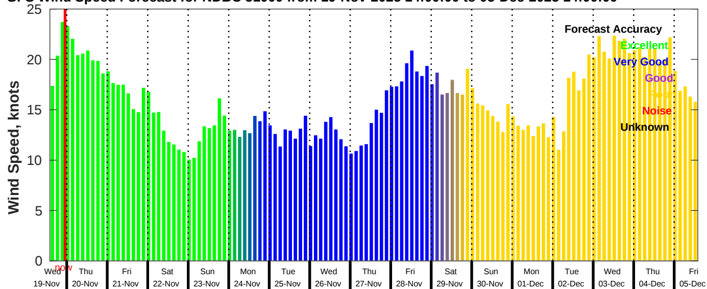
GFS Wind Speed Forecast for NDBC 51000 from 19-Nov-2025 14:00:00 to 05-Dec-2025 14:00:00
